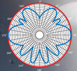
Typical Ringo Ranger
